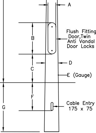
DETAIL "C"
