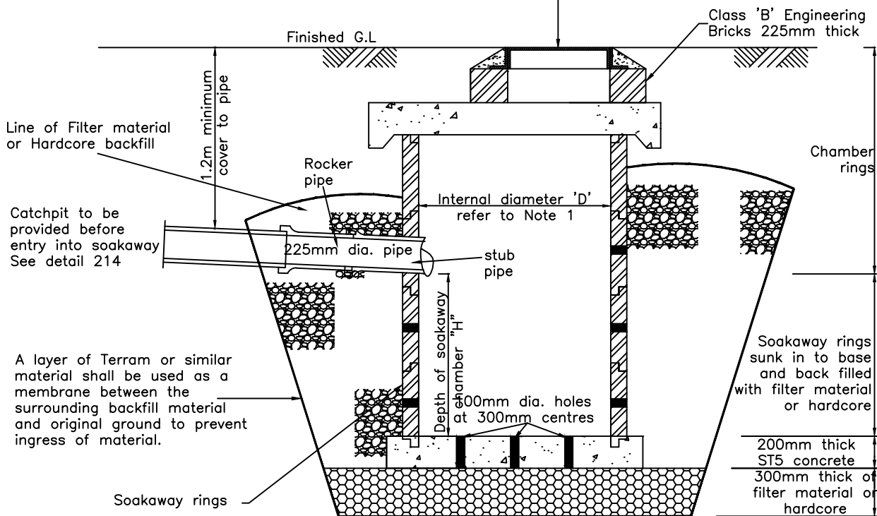
TYPICAL SOAKAWAY
