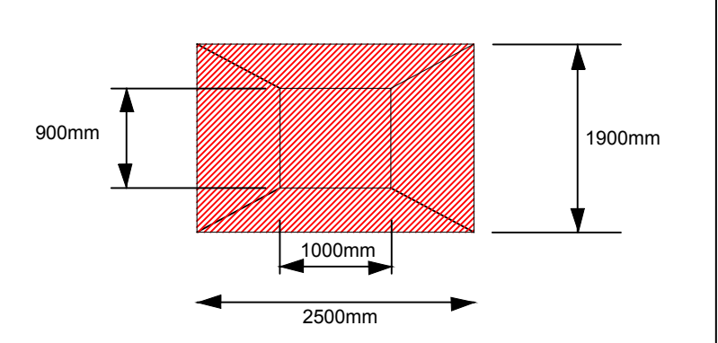
DETAIL B - SPEED CUSHION DETAIL - 2 OR 3 CUSHIONS POSITIONED AT THE LOCATIONS SHOWN - NUMBER OF CUSHIONS IS GOVERNED BY ROAD WIDTH
